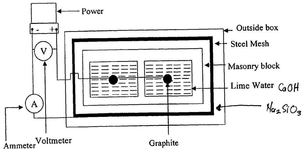
Figure 6. Top view of the block
