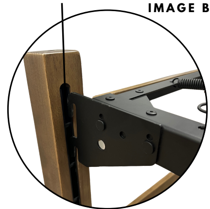
C-CHANNEL WITH PINS
